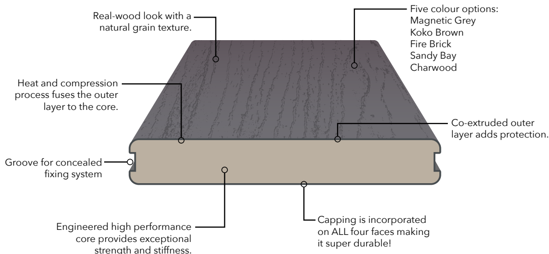
SQUARE PROFILE
