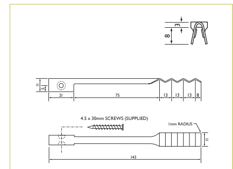
SHERIFF VENEER TIES – MEDIUM DUTY Suits 50mm cavity between brickwork and timber frame.
