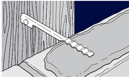
Light Duty Side Fixing Sheriff Veneer Tie for 50mm cavities (with nail)
