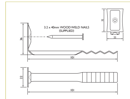
SHERIFF VENEER TIES – LIGHT DUTY Suits 50mm cavity between brickwork and timber frame.
