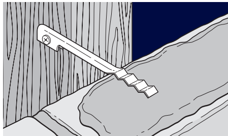
Medium Duty Side Fixing Sheriff Veneer Tie for 50mm cavities (with screw)
