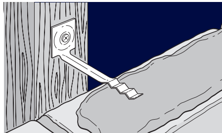
Medium Duty Face Fixing Sheriff Veneer Tie for 50mm cavities (with screw)
