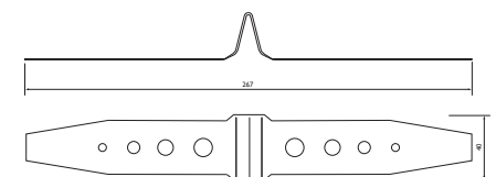
EXPANSION TIES For masonry walls (A.A.C block).
