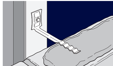
Light Duty Isolation Coated Stainless Steel Face Fix Tie + Hex Screw To Suit .75mm Thick Steel Frame
