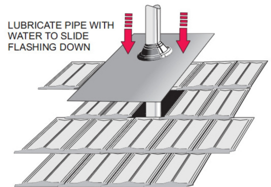
ENSURE ANTI CAPILLARY FOLD IS NOT DEFORMED AT TOP
