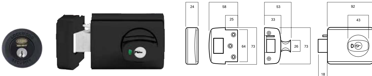
Exterior Cylinder
