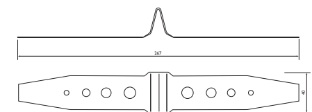
EXPANSION TIES For masonry walls (A.A.C block).
