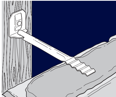
Tremor Veneer Tie for 125-200mm cavities – Medium Duty
